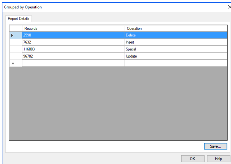
Figure 29 The run report dialog box
