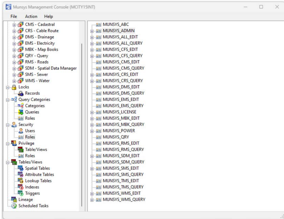
Figure 3 Security tree: roles
