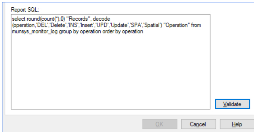
Figure 33 The Report SQL text box
