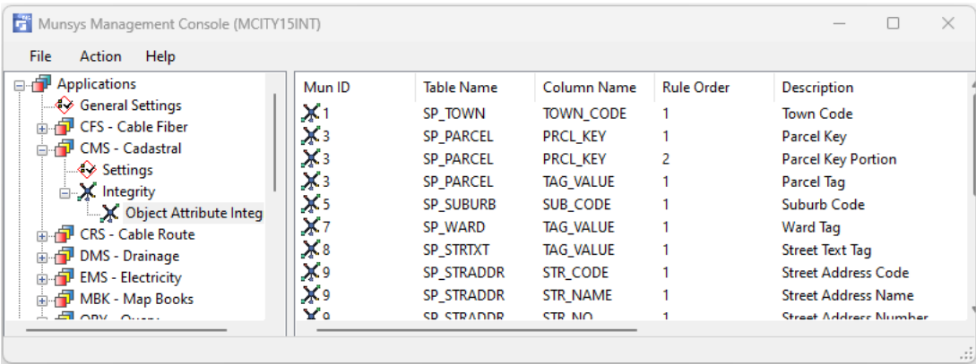
Figure 35 Select Object Attribute Integrity
