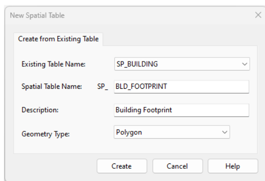
Figure 6 Creating a new spatial table
