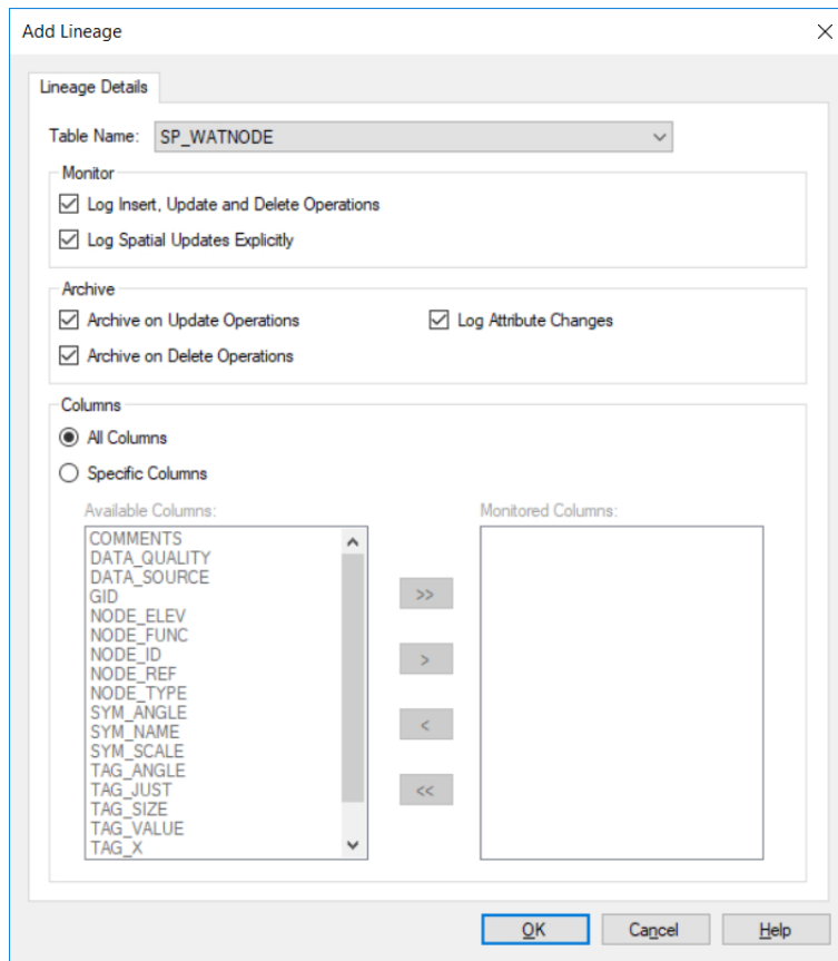
Figure 8 The Add Lineage dialog box
