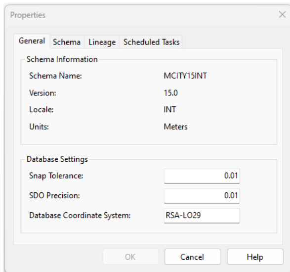
Figure 19 Schema Properties: General
