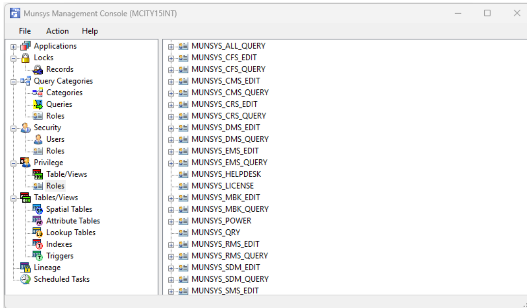
Figure 2 Privilege tree: roles
