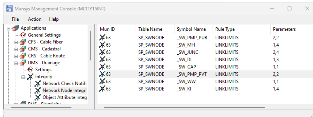
Figure 16 Munsys Management Console: Network Node Integrity
