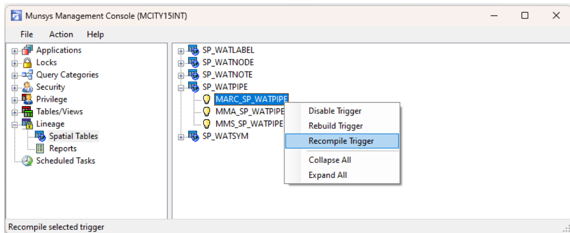
Figure 20 Recompile selected trigger
