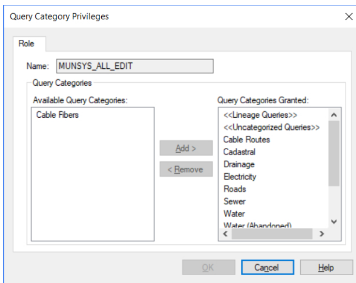
Figure 16 The Query Category Privileges
