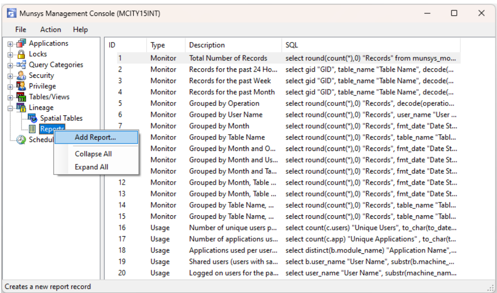
Figure 35 Add Report selection
