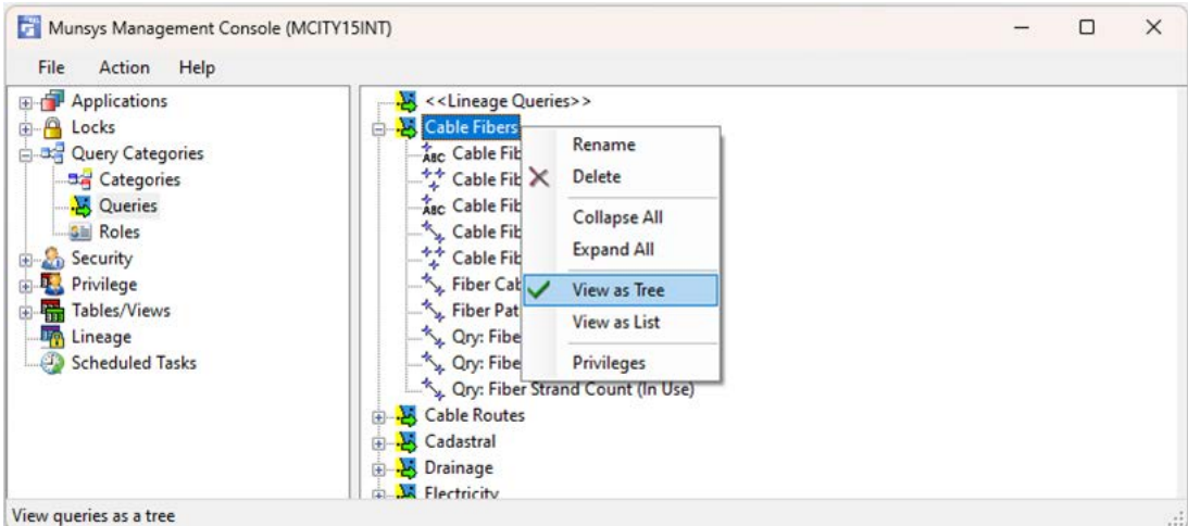
Figure 7 View queries as tree
