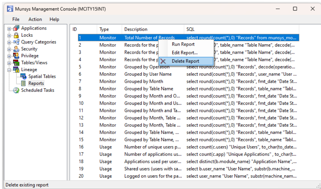
Figure 38 Delete Report selection
