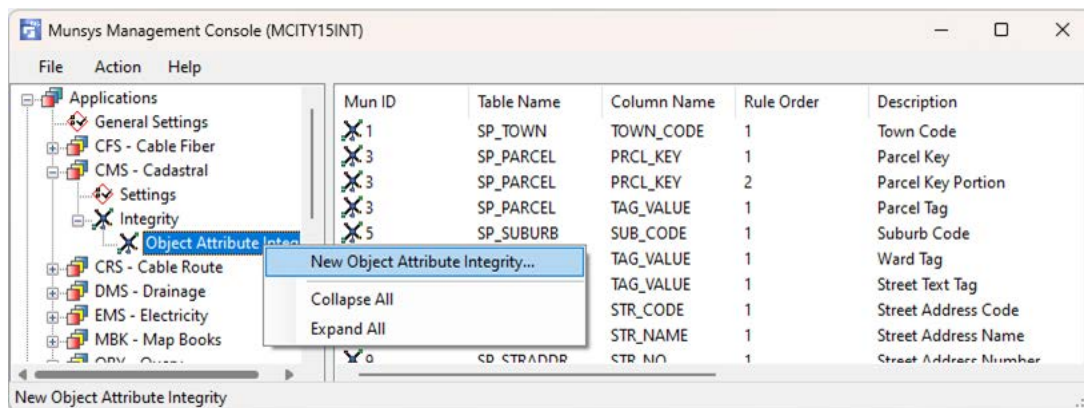
Figure 30 Create new Object Attribute Integrity
