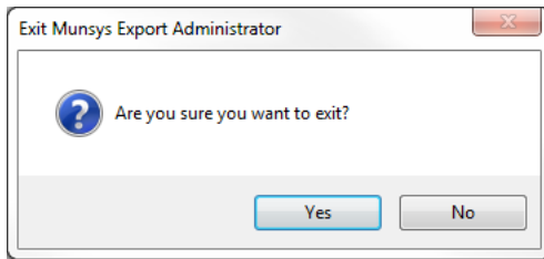
Figure 23 Exit message
